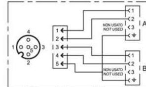
CONNECTOR M12x1 CONNECTION SCHEME
